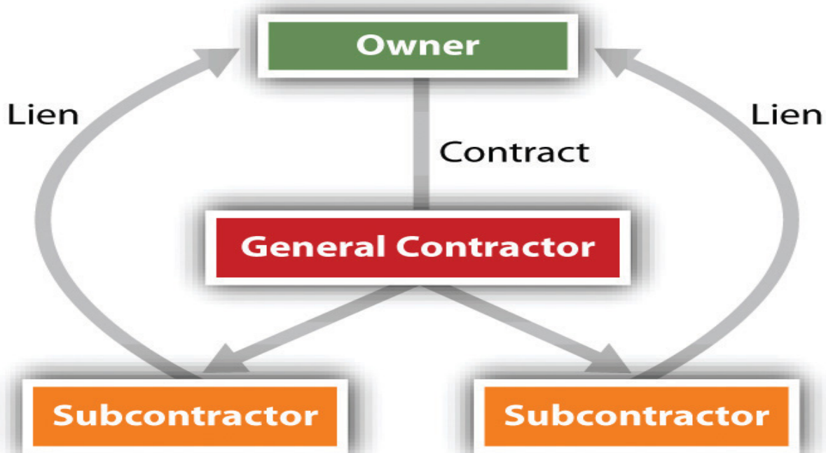
Figure 11.5 Subcontractors’ Lien
